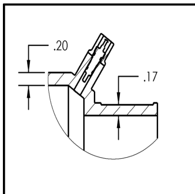
Molded-in Air Valve detail
