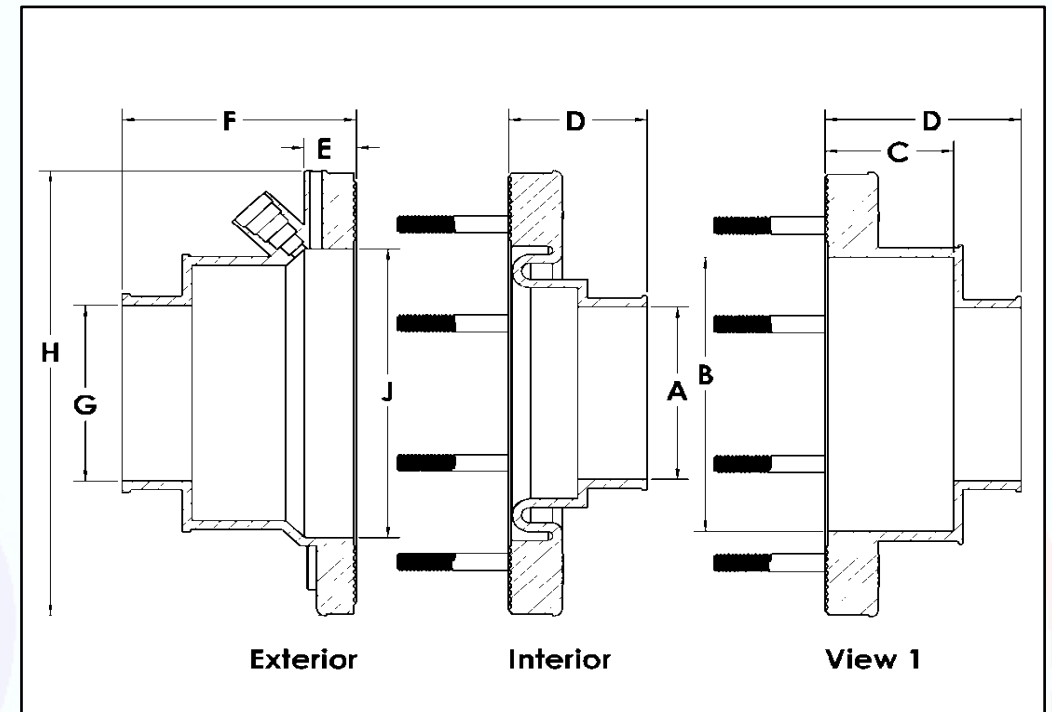
Inverted Studed Filled Penetration Fitting
